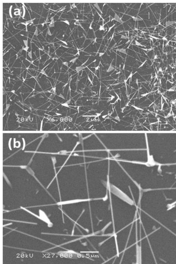
Fig. 1: (a) low and (b) high magnifications SEM images of ZnO nanowires, prepared at 750 °C and oxygen flow rate of 20 sccm.
